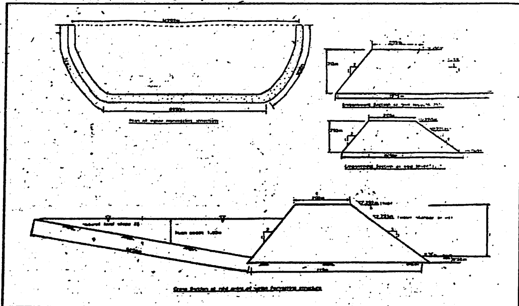
(DESIGN DETAILS OF EARTHEN BUND)
