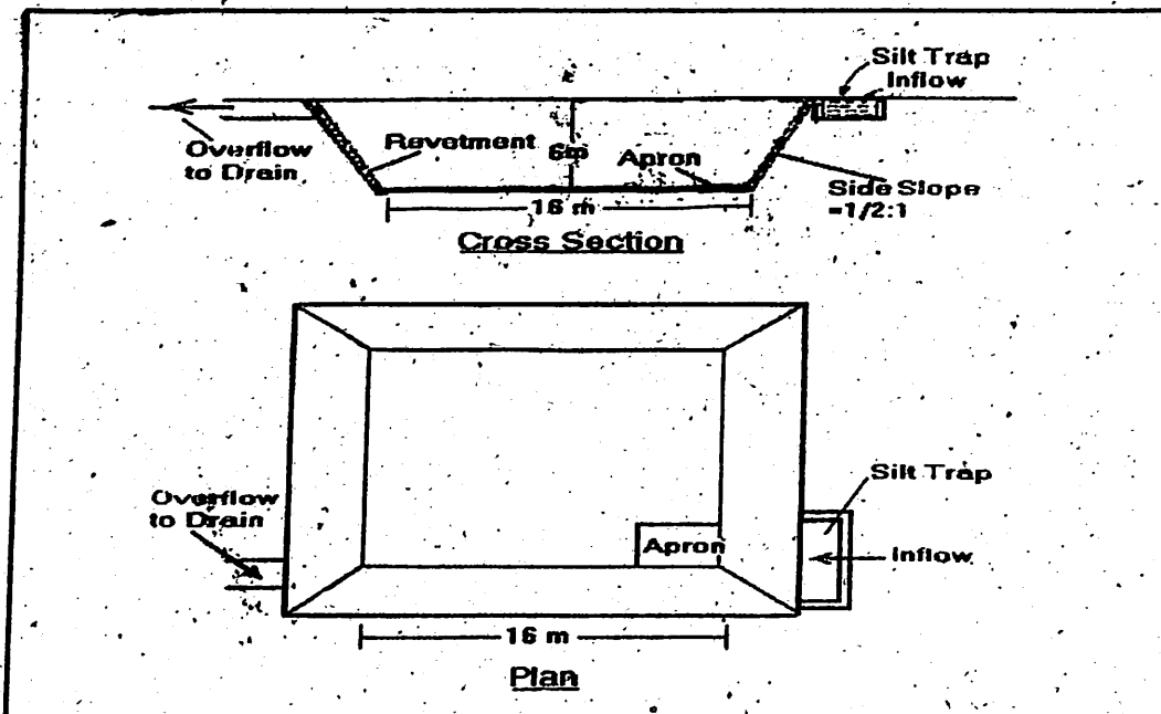
(SCHEMATIC DIAGRAM OF A PERCOLATION TANK- TYPICAL DESIGN)
