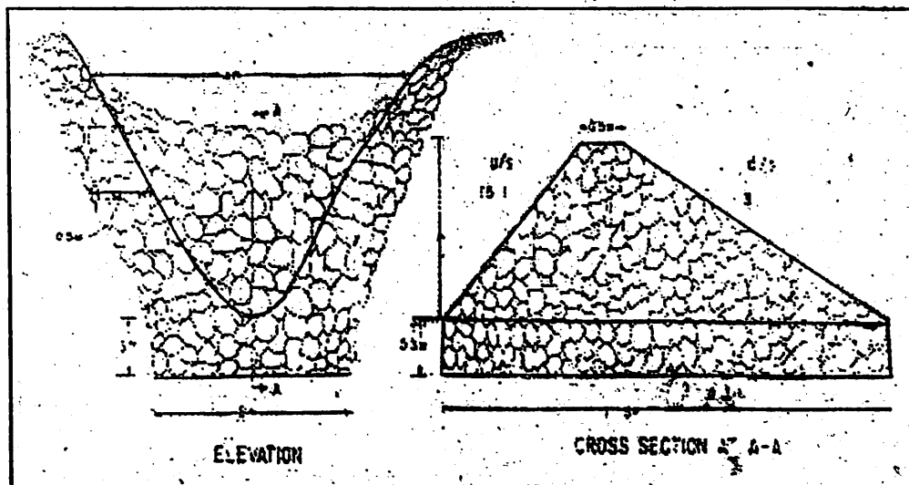
(DESIGN DETAILS OF LOOSE BOULDER CHECK DAM)
